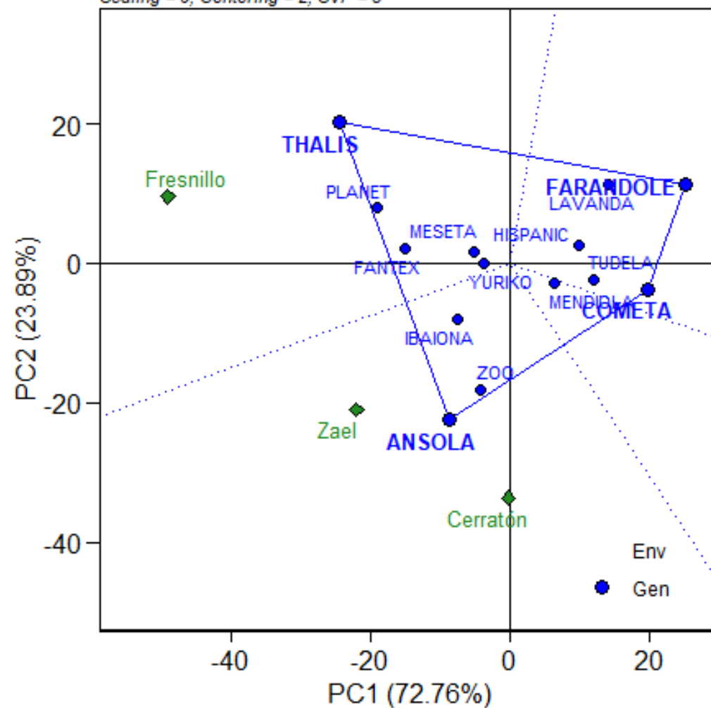
Which-won-where view of the GGE biplot
